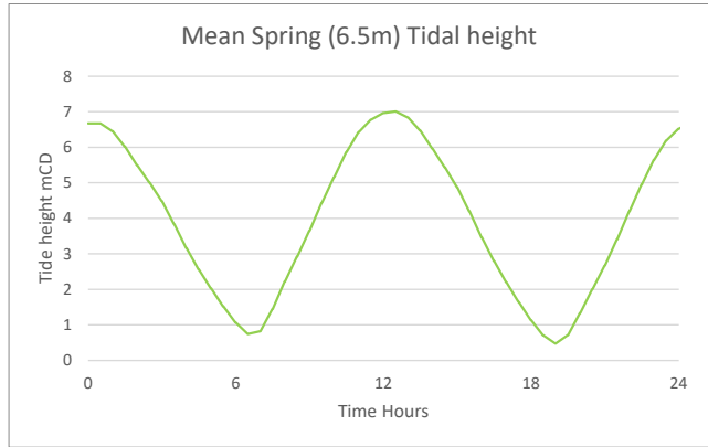
Figure 2.11: Mean spring tidal height as simulated
