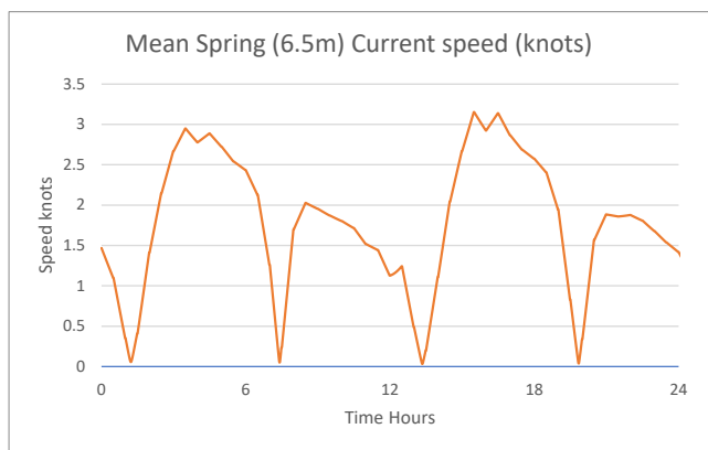
Figure 2.15: Mean spring current speed as simulated
